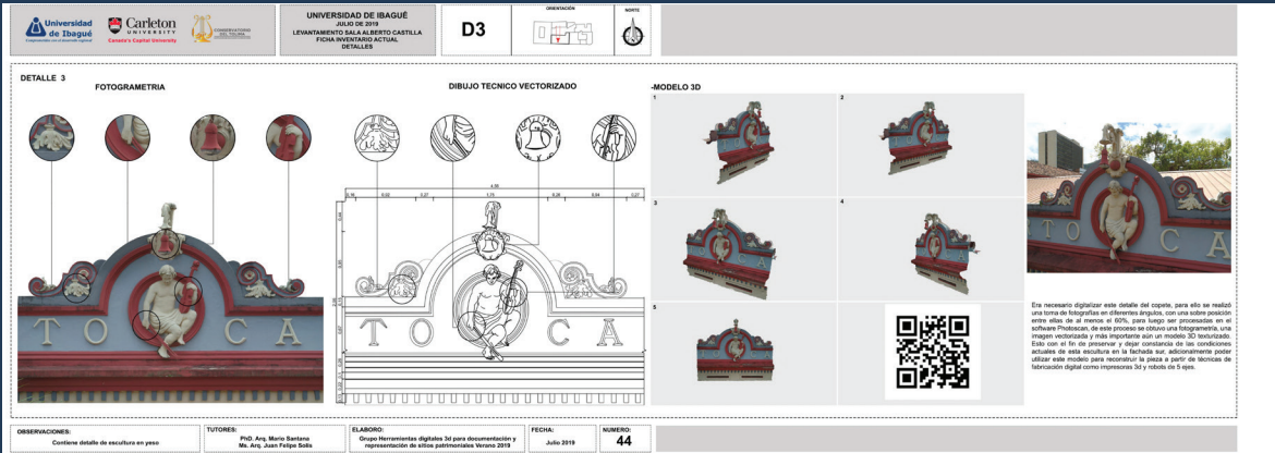
Three-Dimensional Representation of an Architectural Detail in the Alberto Castilla Hall (Colombia). © J. Solís y M. Santana.
